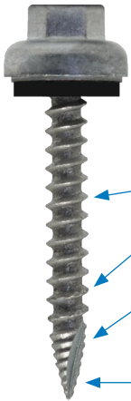
#10-12 ZINC CAP HEAD | 5/16" HWH Washer: .565" Dia. / Aluminum to EPDM
