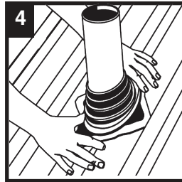
4 Form flashing to roof profile
