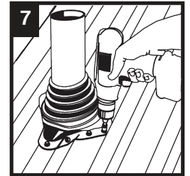
7 Fasten flashing to complete
