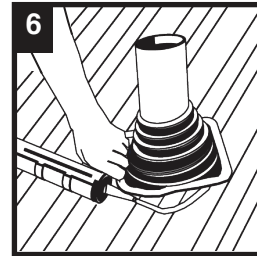
6 Apply Sealant
